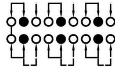
SCHEMATIC (NON-SHORTING)
