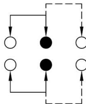
SCHEMATIC (NON-SHORTING)
