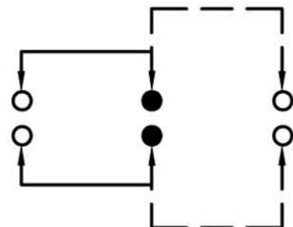
SCHEMATIC(NON-SHORTING)
