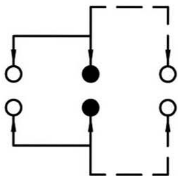
SCHEMATIC (NON-SHORTING)
