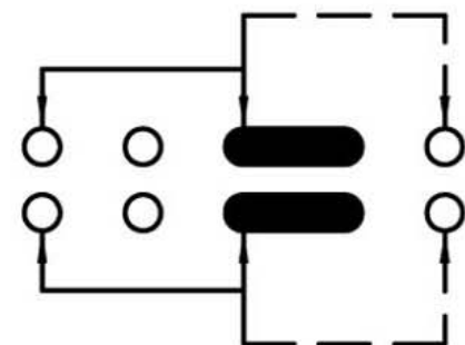
SCHEMATIC(NON-SHORTING)
