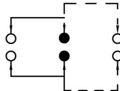
SCHEMATIC (NON-SHORTING)
