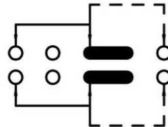
SCHEMATIC (NON-SHORTING)
