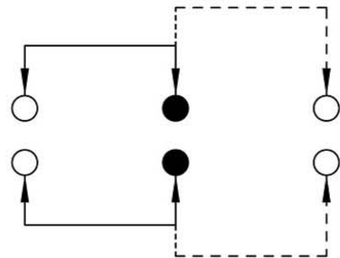
SCHEMATIC (NON-SHORTING)
