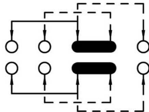
SCHEMATIC (SHORTING)
