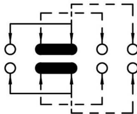
SCHEMATIC (SHORTING)
