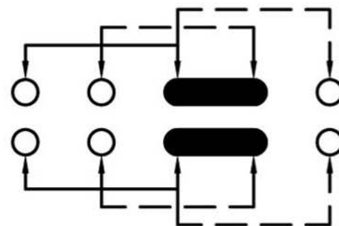
SCHEMATIC (SHORTING)
