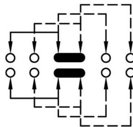
SCHEMATIC (SHORTING)
