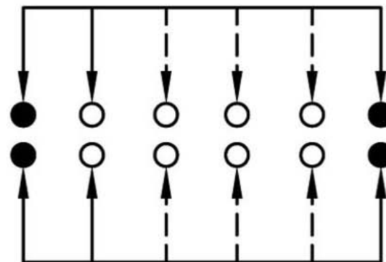
SCHEMATIC (NON-SHORTING)
