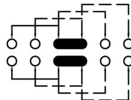
SCHEMATIC (SHORTING)
