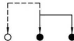
SCHEMATIC (NON-SHORTING)
