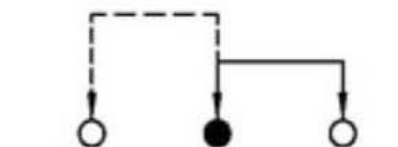
SCHEMATIC (NON-SHORTING)
