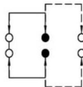
SCHEMATIC (NON-SHORTING)
