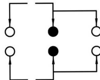
SCHEMATIC (NON-SHORTING)
