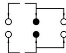
SCHEMATIC (NON-SHORTING)
