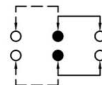
SCHEMATIC (NON-SHORTING)
