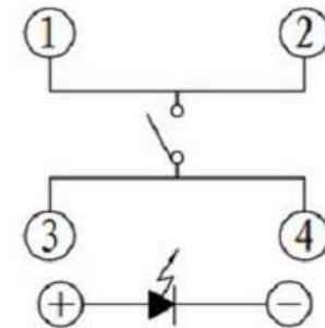
SCHEMATIC
