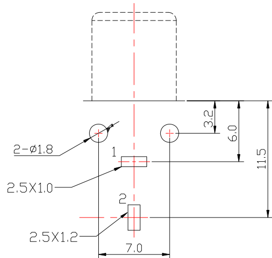
PCB HOLES DIAGRAM TOP VIEW
