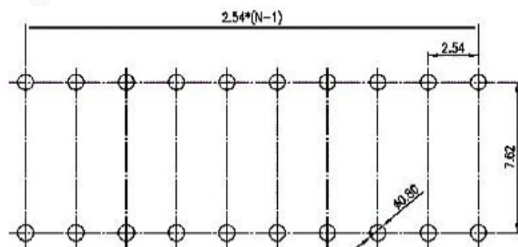
RECOMMENDED P.C.B. LAYOUT (UNIT: MM)
