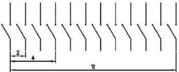
RECOMMENDED P.C.B. LAYOUT (TOP VIEW) [Schematic]
