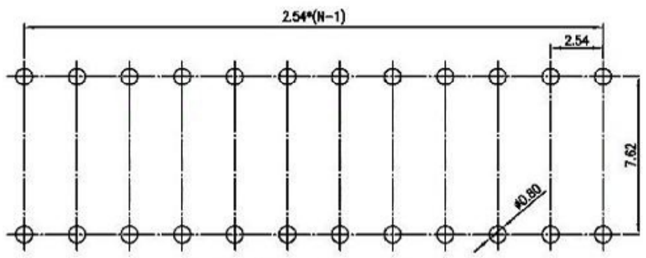
RECOMMENDED P.C.B. LAYOUT (TOP VIEW) [Schematic]
