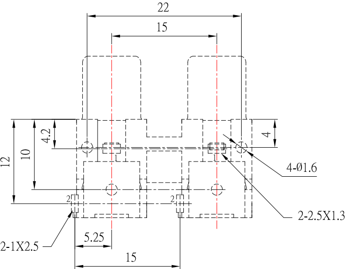
PCB HOLES DIAGRAM BOTTOM VIEW
