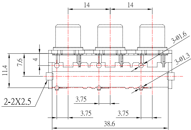
PCB HOLES DIAGRAM BOTTOM VIEW
