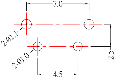
P.C.B LAYOUT MOUNTING PATTERN TOP VIEW
