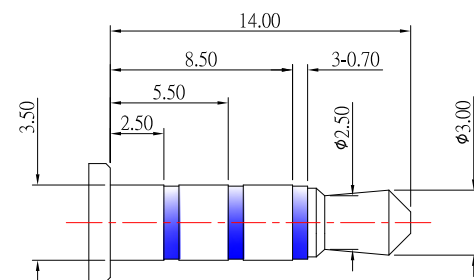
(3.5mm 4 POLE PLUG DETAIL DRAWING)
