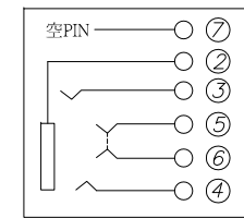
SCHEMATIC
