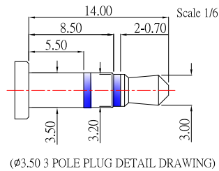
(ø3.50 3 POLE PLUG DETAIL DRAWING)
