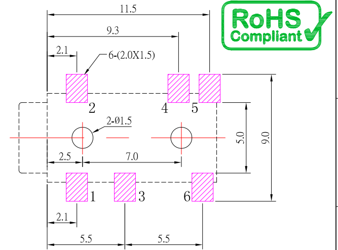
P.C.B LAYOUT TOP VIEW SCHEMATIC
