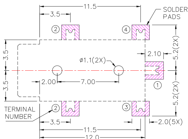
RECOMMENDED SOLDER PAD LAYOUT (TOP VIEW)
