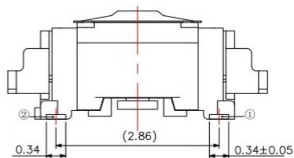
Actuator cross section (Section C-C)
