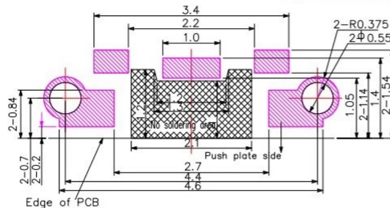
PCB LAYOUT
