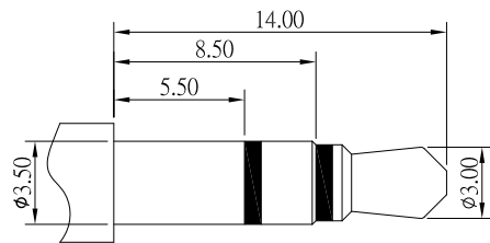
ø3.50mm 3 POLE PLUG
