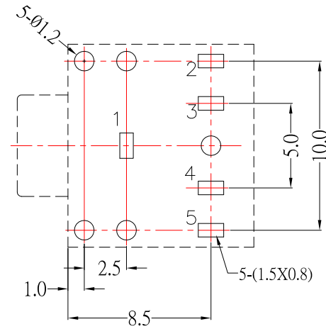
P.C.B LAYOUT MOUNTING PATTERN (TOP VIEW)
