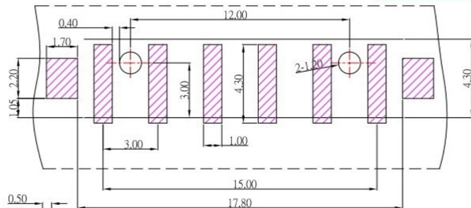
RECOMMEND PCB LAYOUT
