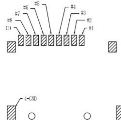
PIN ASSIGNMENT
