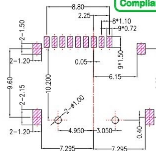
PCB LAYOYT
