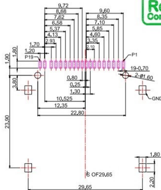
RECOMMEND PCB LAYOUT
