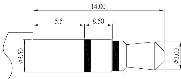
03.50mm 3 POLE PLUG
