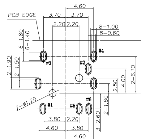
RECOMMENDED P.C.B LAYOUT TOP VIEW (TOLRANCE:±0.05)
