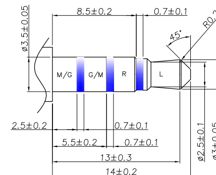
Matching Plug
