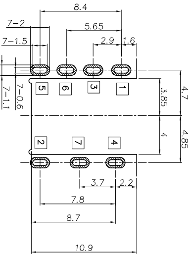
RECOMMENDED P.C.B LAYOUT(≠1.0mm) TOP VIEW (TOLERANCE: ±0.05)
