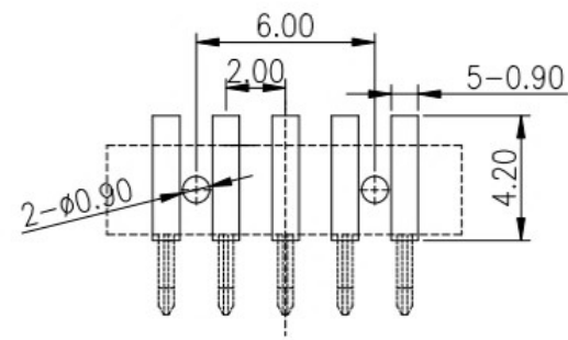
RECOMMENDED P.C.B LAYOUT TOP VIEW (.XX±0.05)
