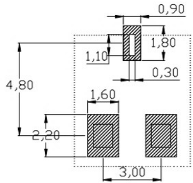
RECOMMENDED PCB LAYOUT TOP VIEW (.XX±0.05)
