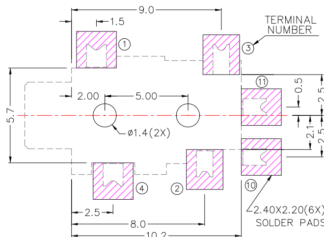
RECOMMENDED SOLDER PAD LAYOUT
