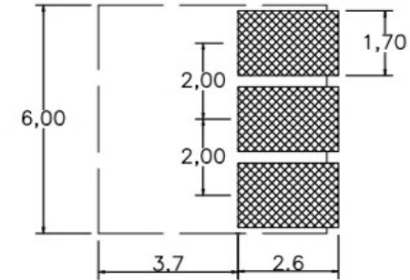
RECOMMENDED PCB LAYOUT TOP VIEW(. XX±0.05)
