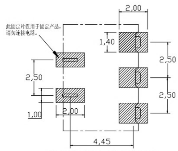
RECOMMENDED PCB LAYOUT TOP VIEW(.XX±0.05)
