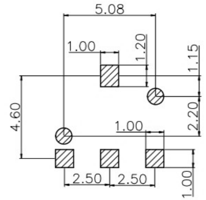
PCB Layout
