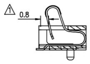
VIEW A-A'
