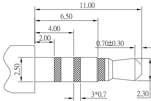
Ø2.50mm 4 POLE PLUG
