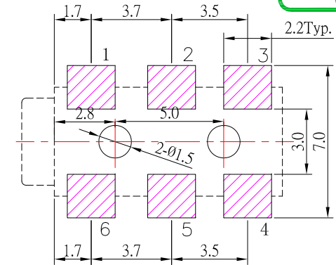
P.C.B LAYOUT MOUNTING PATTERN (TOP VIEW)
