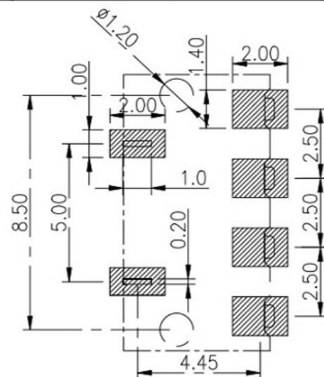
RECOMMENDED PCB LAYOUT TOP VIEW (.XX±0.05)
